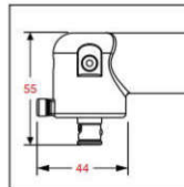
OP-311LHA F Rear exhaust 後排氣
