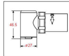
OP-302L90 F 360° Rotate side exhaust 360°調整側排氣
