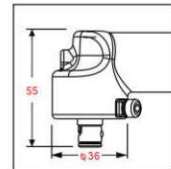
OP-310LHA F Side exhaust 側排氣
